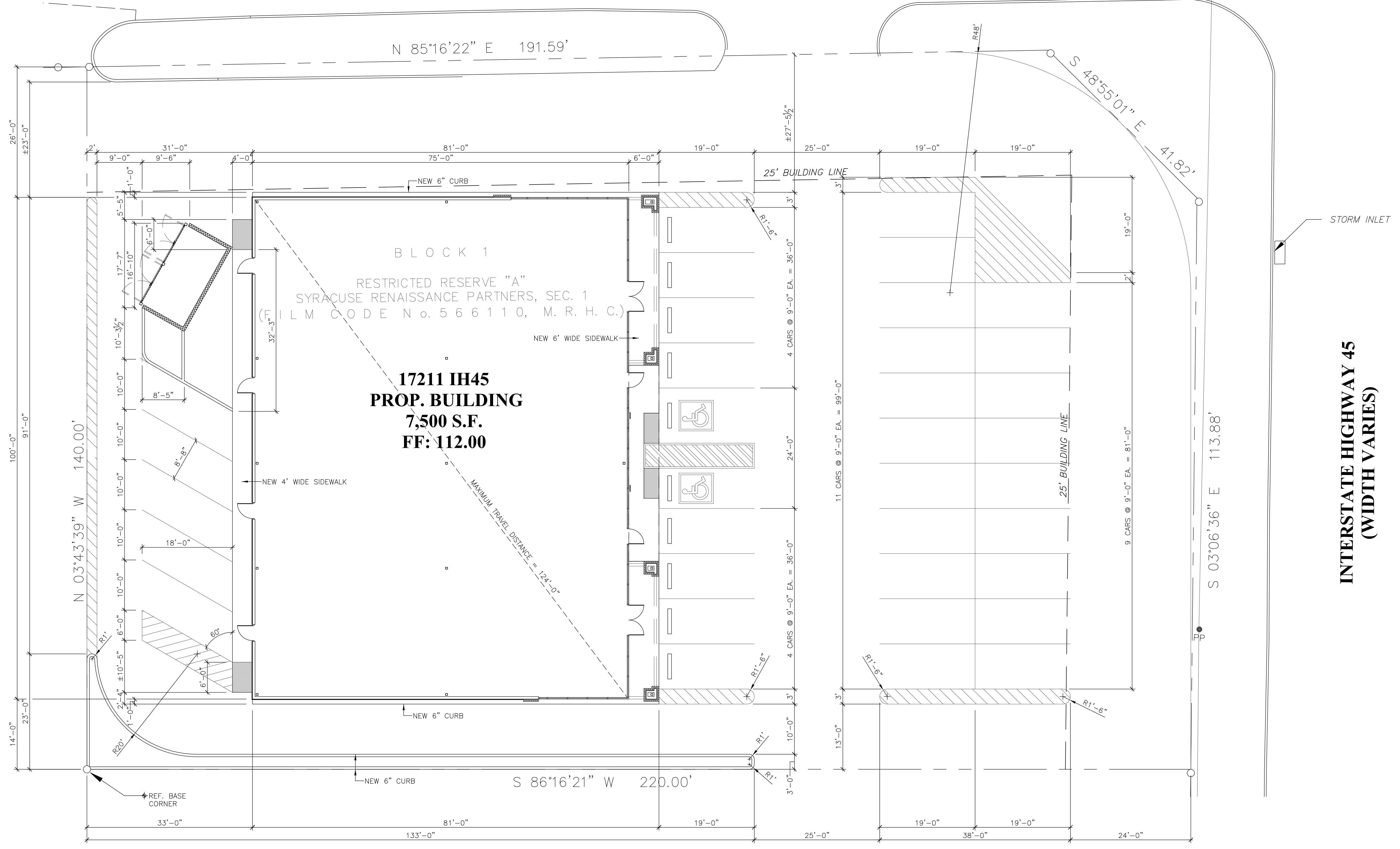
1 ARCHITECTURAL SITE PLAN A1.1 1" = 10'-0"
